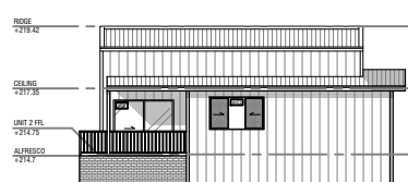
EASTERN ELEVATION NTS
