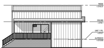
NORTHERN ELEVATION NTS
