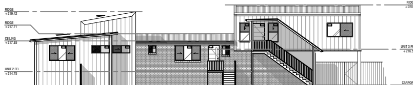
NORTHERN ELEVATION NTS
