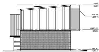
WESTERN ELEVATION NTS
