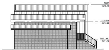
SOUTHERN ELEVATION NTS
